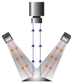
IDBA Series Bar Lights used individually or in combination for bright or dark field illumination.
